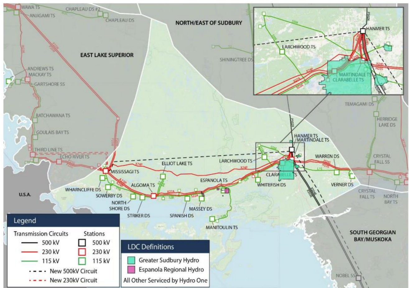
Figure 1 | Sudbury Algoma Electricity Infrastructure
