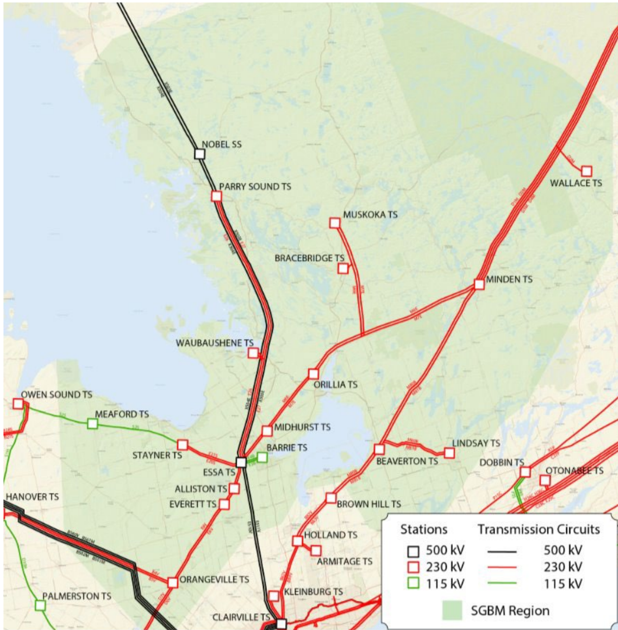
Figure 1 | South Georgian Bay/Muskoka Electricity Infrastructure
