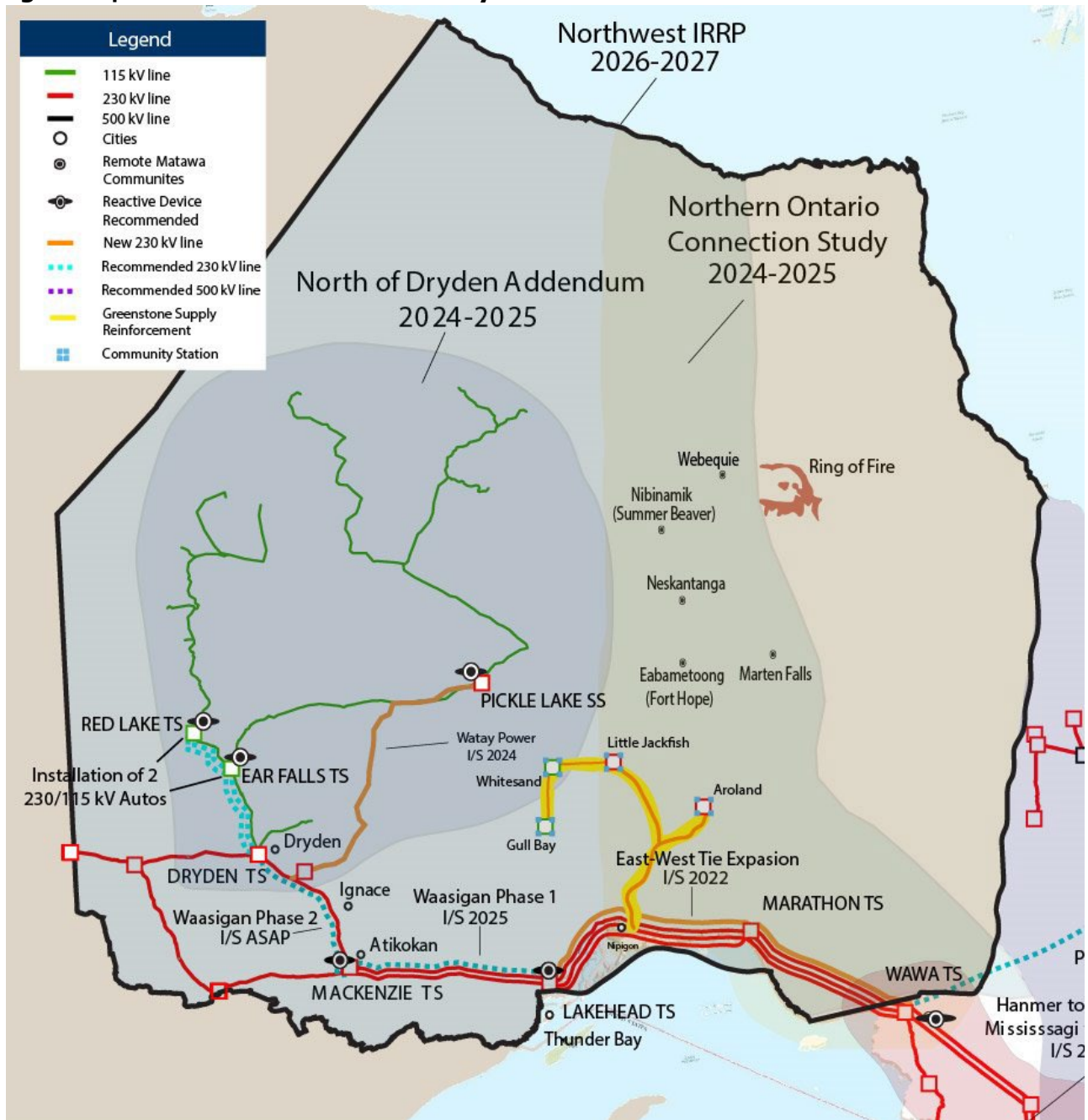
Figure 1 | Northwest Ontario Electricity Infrastructure
