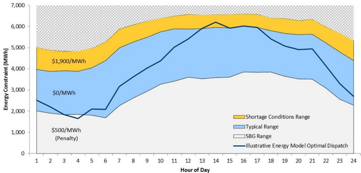
Figure 5-2 | Hydroelectric Solution for a Particular Weekday vs. Hourly and Daily Energy Constraints
