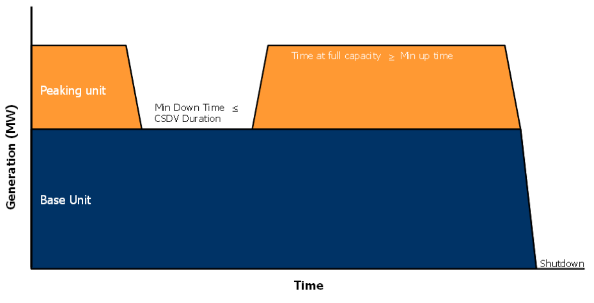
Figure 5-1 | Nuclear Manoeuvring Unit Dispatch Illustration
