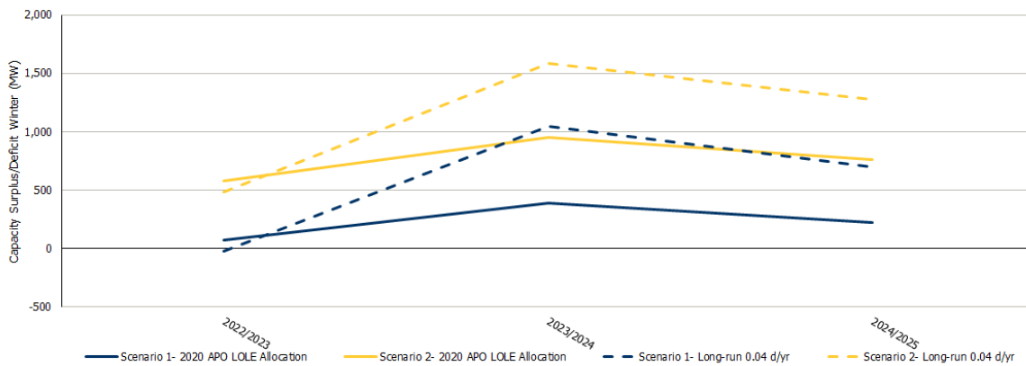
Figure 6 | Impact of 2020 APO LOLE Allocation vs. Long-Run Assumption, Winter
