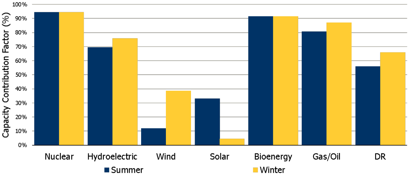
Figure 2 | Summer and Winter Capacity Contribution
