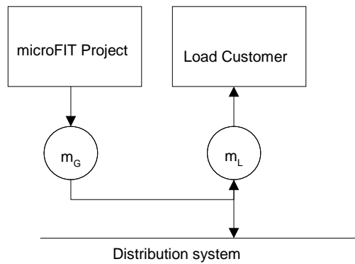
Figure 2 – Indirectly connected microFIT Project (in parallel)
