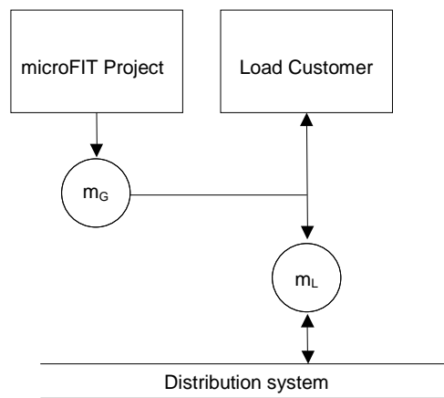
Figure 3 – Indirectly connected microFIT Project (in series)
