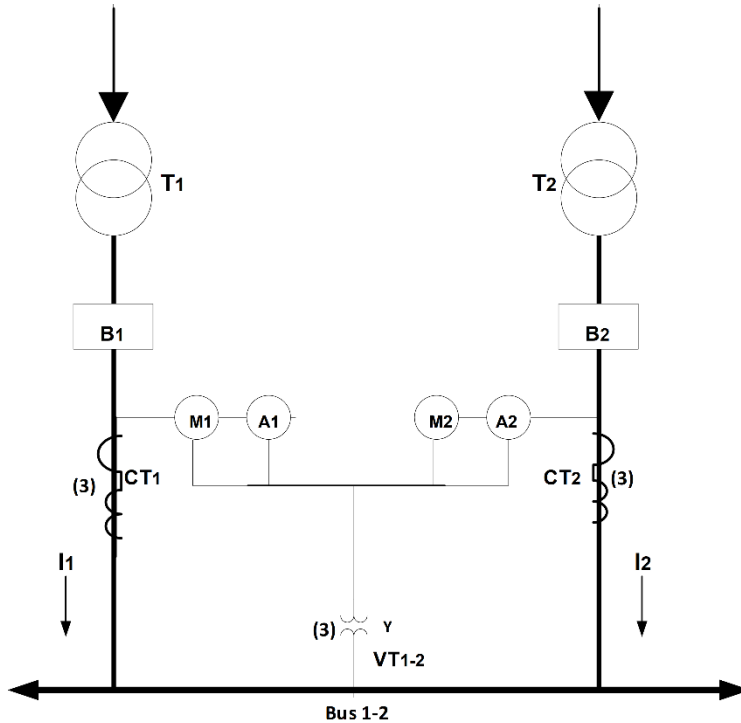
Figure D-2: Six current transformers and Three voltage transformers in a Metering Installation for Two Equally-Loaded, Equivalent Transformers T 1 and T 2 , Connected to a Common Load Bus
