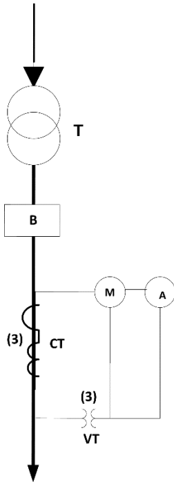
Figure D–1: Three Current Transformers and Three Voltage Transformers in a Metering Installation (Single Circuit)
