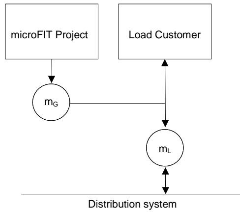
Figure 2 – Indirectly connected microFIT Project (in parallel)
