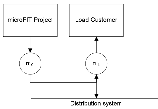
Figure 2a – Indirectly connected microFIT Project (in parallel)
