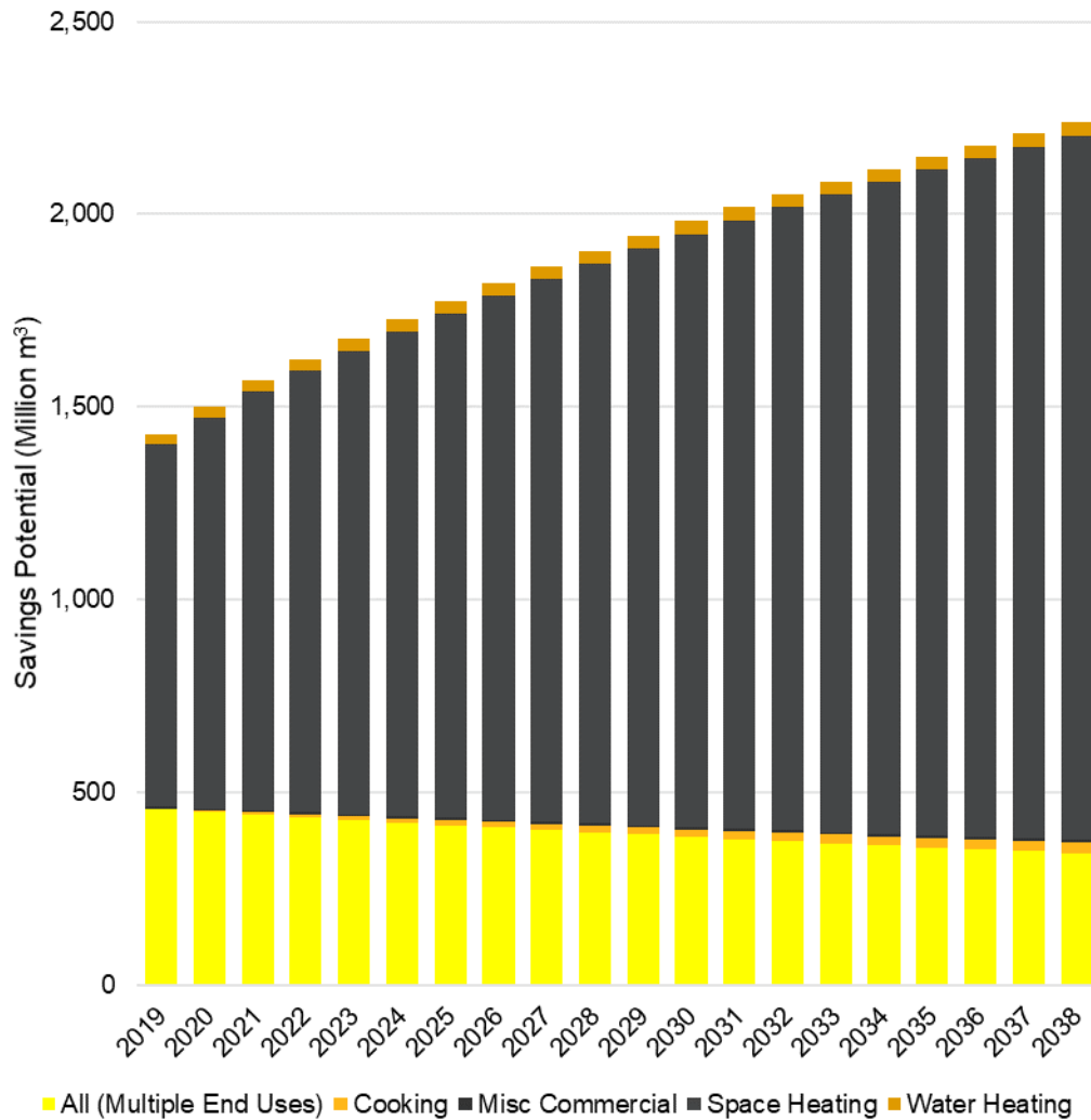
Figure 5-18. Commercial Natural Gas Energy Technical Potential by End Use (Million m 3 )
